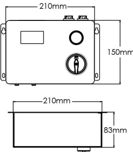
Controller box
